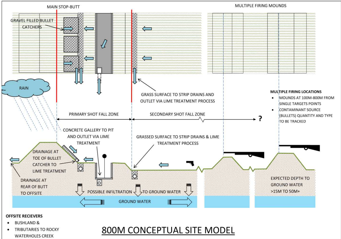
FIGURE 6: 800m Range: Conceptual Site Model (CSM)
